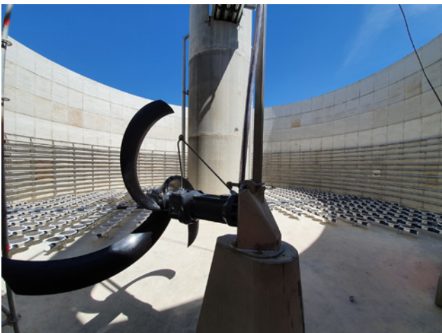
The annamox process uses 480 disc diffusers supplied by two HST 2500 turbocompressors
